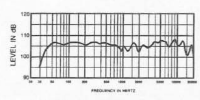
FIGURE 5 - MTH-2/94A Axial Frequency Response using Recommended Crossover, Equalization, Time Delay and MTL-2 Low-Frequency System
